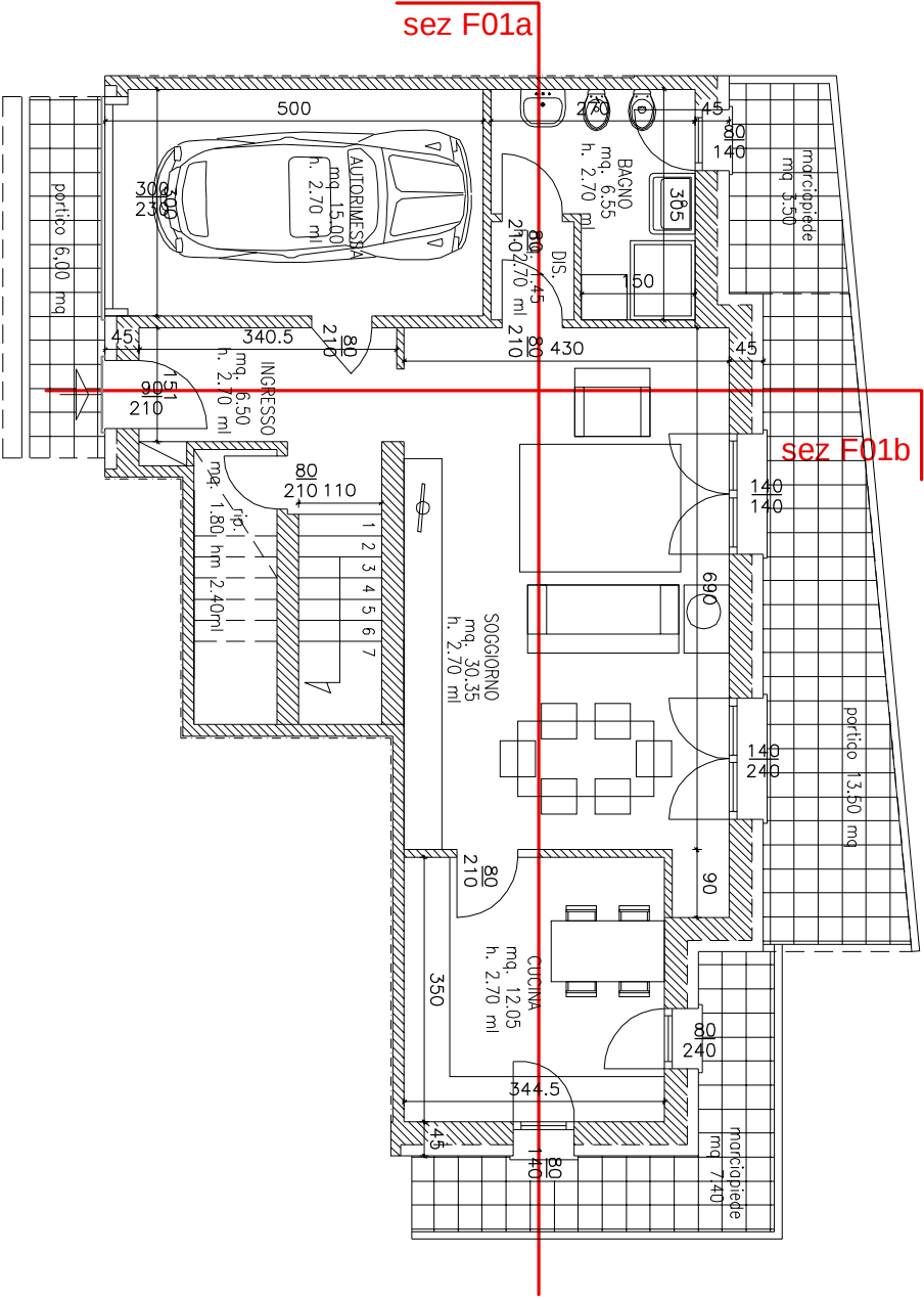
PIANO TERRA
